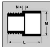
MALE ADAPTER (Mipt x Slip)
