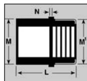
FEMALE ADAPTER (Fipt x Slip) Stainless Steel Reinforced
