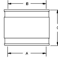
SIZE-ON-SIZE
