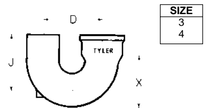
SINGLE HUB RETURN BEND
