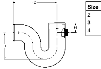
RUNNING TRAP W/4" SINGLE VENT
