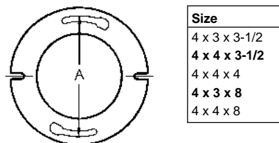
9-480 CLOSET FLANGE (Slot & Notch)
