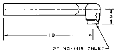
2" NO-HUB INLET
