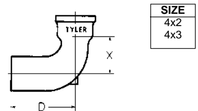
QUARTER BEND REDUCING
