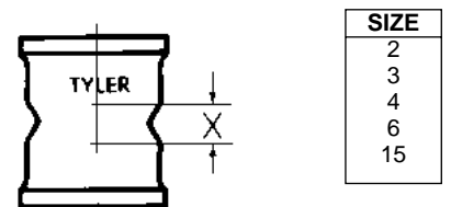
DOUBLE HUB FITTING
