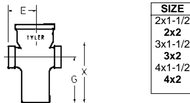
TWO-WAY CLEANOUT
