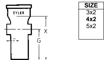
DOUBLE HUB FITTING
