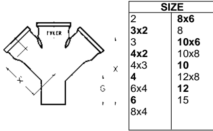
DOUBLE WYE
