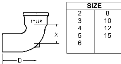
SIXTEENTH BEND
