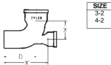
QUARTER BENDING W/Low Heel Inlet
