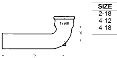
LONG QUARTER BEND
