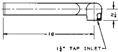
1 1/2" TAP INLET
